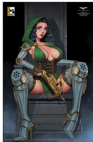
Dravacus - RHESII
